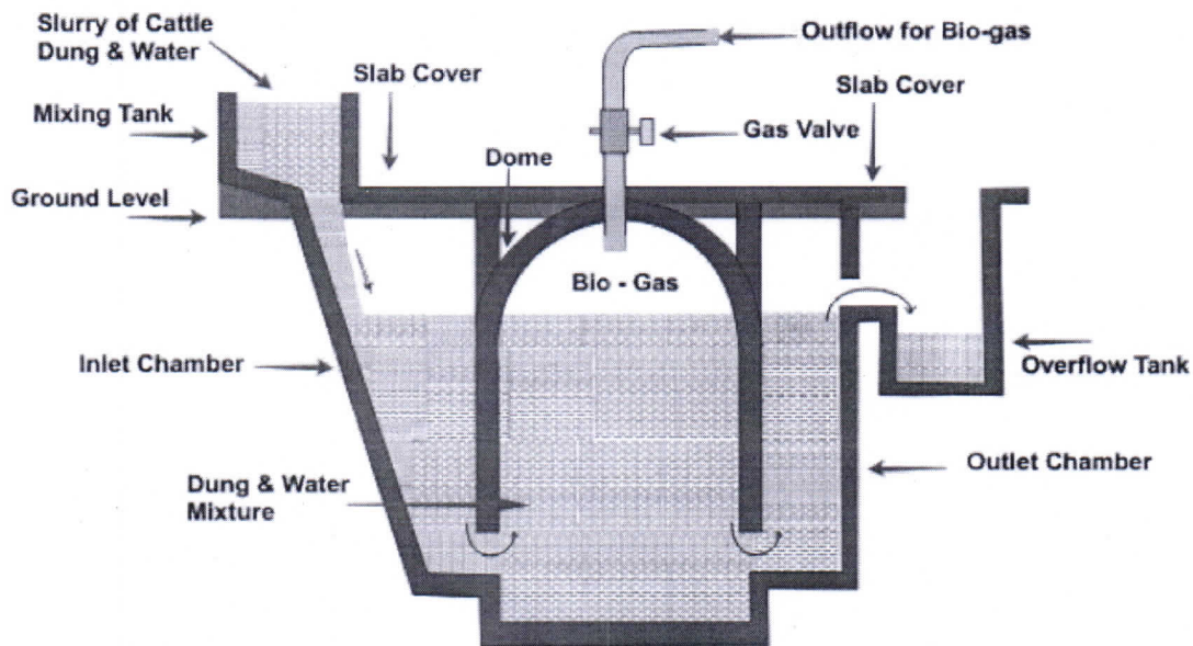
Fixed Dome type Bio-gas Plant
